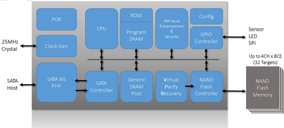
[Figure 1-1] SSD Functional Block Diagram
