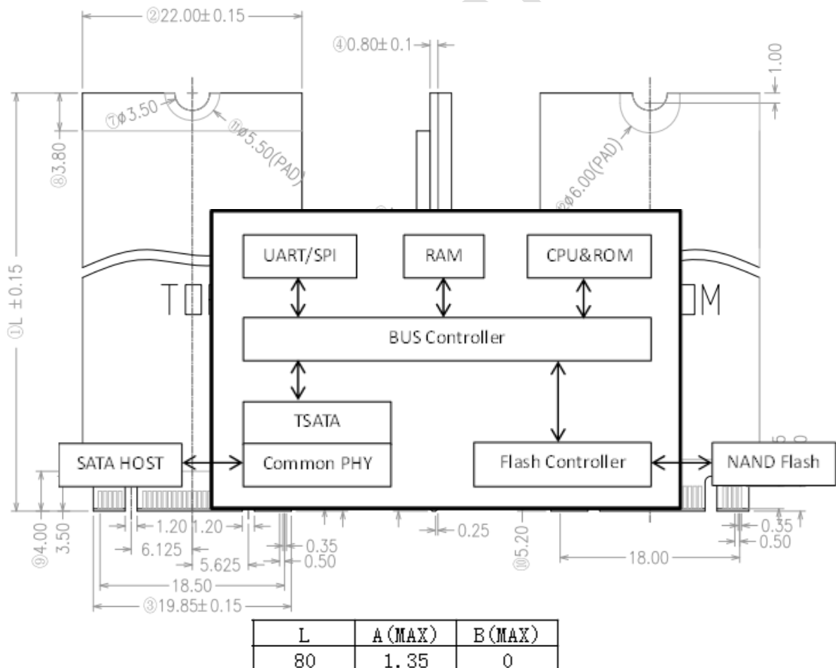
[Figure 2-1] M.2 2280 SSD Physical dimension
