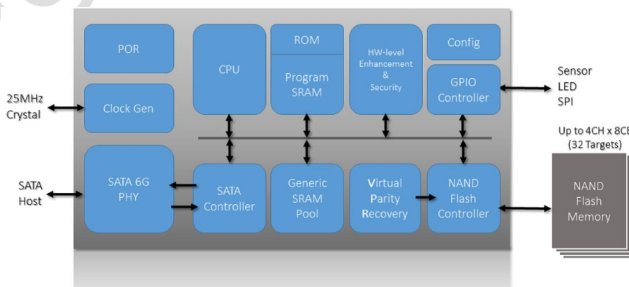
[Figure 1-1] SSD Functional Block Diagram
