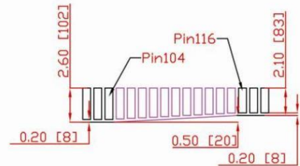
Detail D
